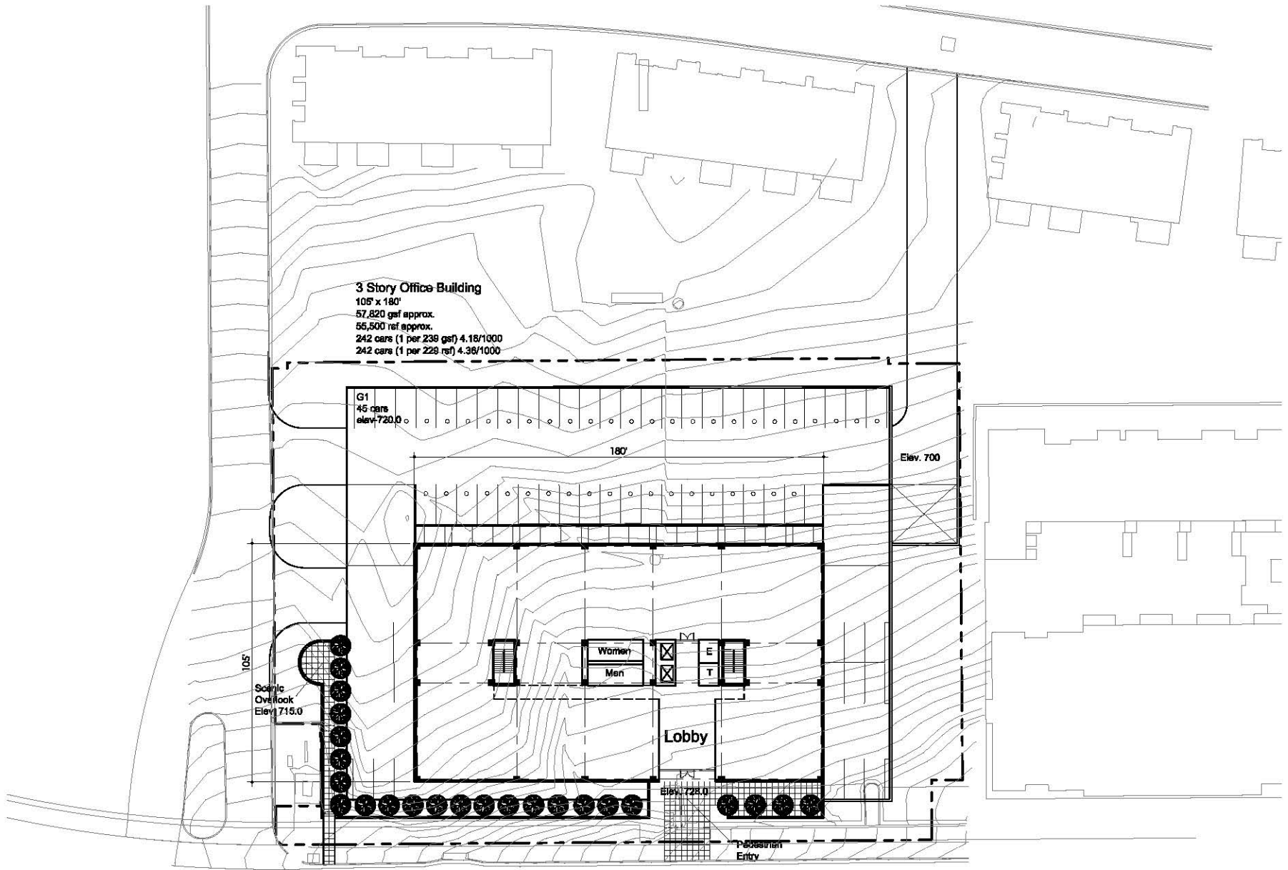
1st Floor Site Plan
